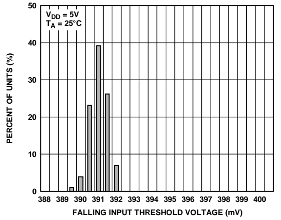
Figure 8. Distribution of Falling Input Threshold Voltage
